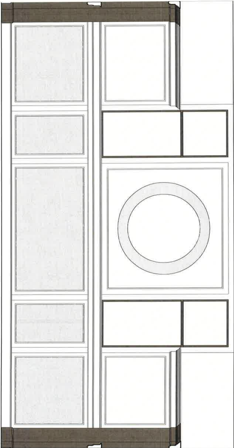
① NORTH ELEVATION 3/8" = 1'-0"
